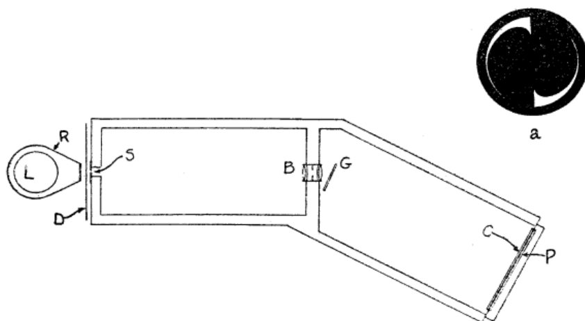
FIG. 2.—Diagram of spectrograph
