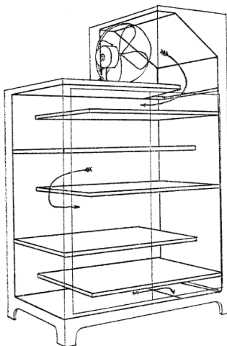
FIG. 22.—Drying cabinet
