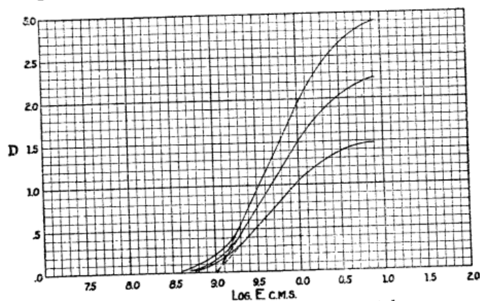
FIG. 19.—Spectrum process plate, untreated
