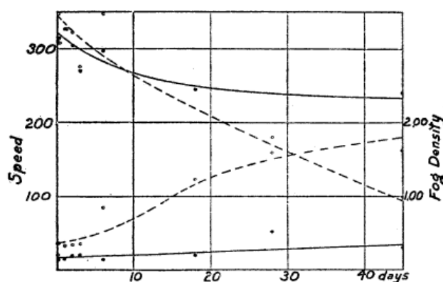
FIG. 8.—Keeping tests on plates sensitized with pinacyanol
