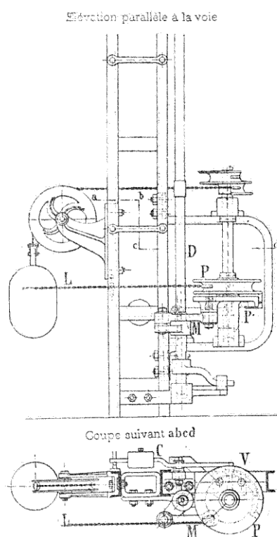
FIG. 101. — Verrou de signal Forest.
