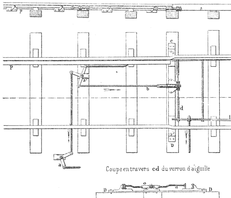
Fig. 109. — Verrou Saxby.
