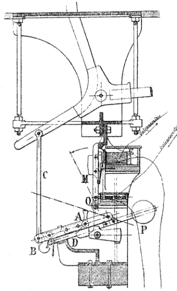
Fig. 199. — Electric slot signal.
