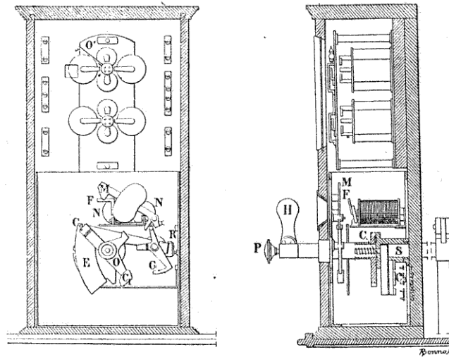
Fig. 244. — Block Hodgson.
