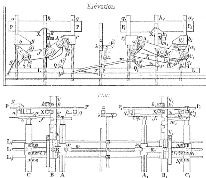
FIG. 198. — Bouton de direction.
