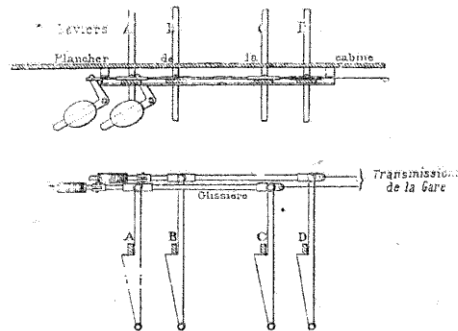
Fig. 178. — Safety-lock.
