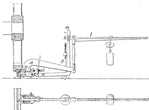
FIG. 294. — Balance Erard.
