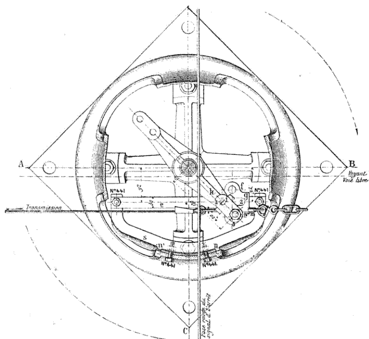
FIG. 102. — Calage Marcelet.
