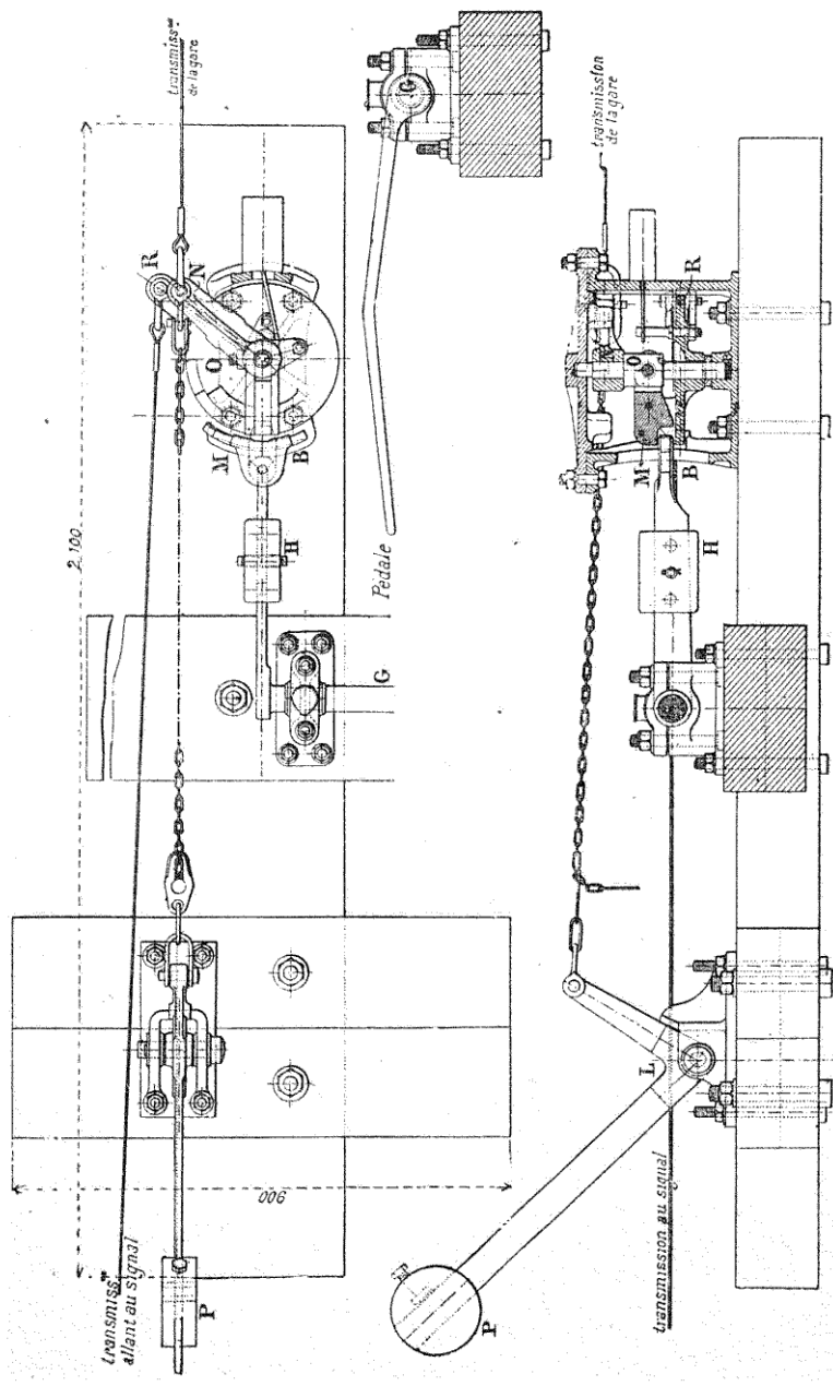
Fig. 88. — Pedale Aubine.
