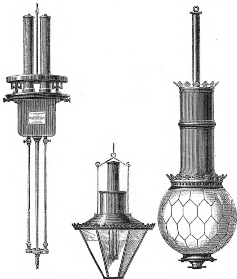
Lampes Brush.
