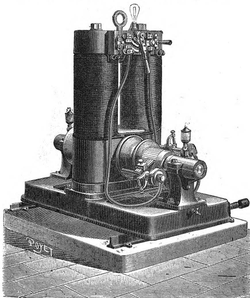
Machine Edison.
