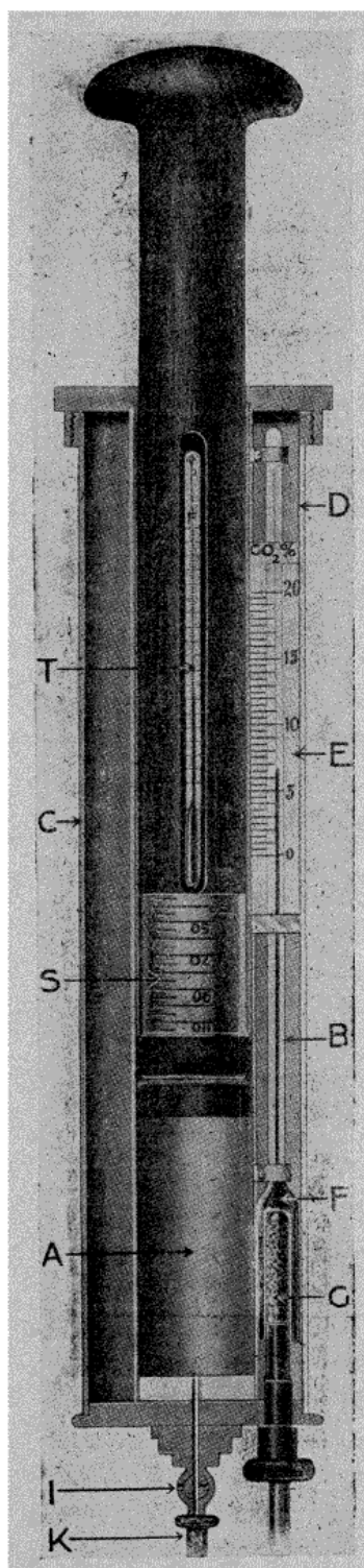
Fig. 9. — ThermoSCOPE Usco.
