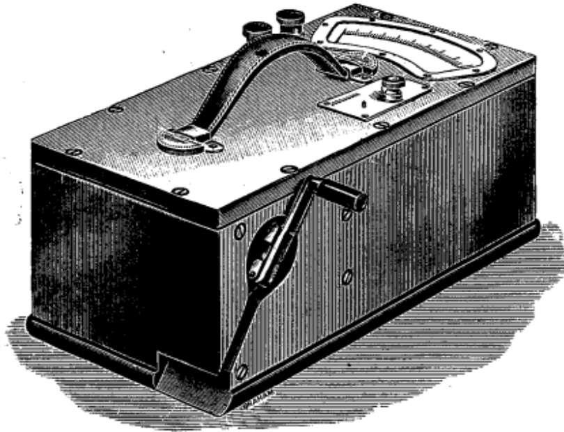
Ohmer Insulation Testing Set. FIG. 17.
