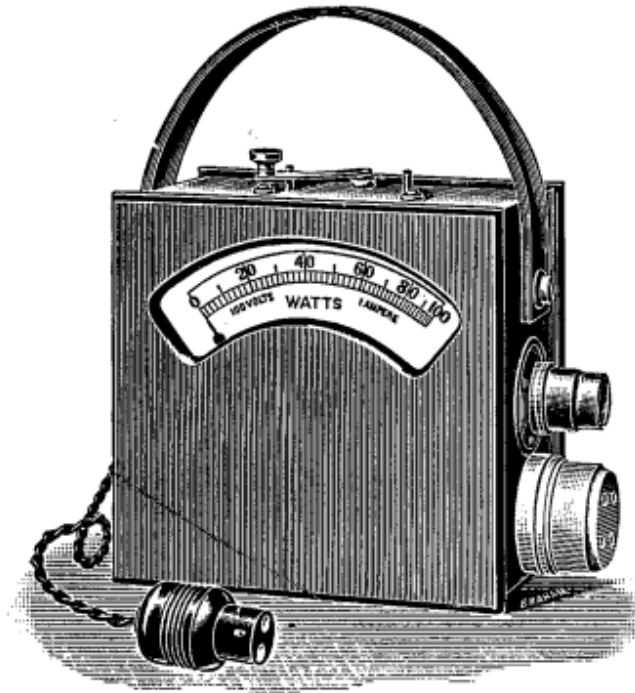
Lamp Testing Wattmeter. FIG. 4.
