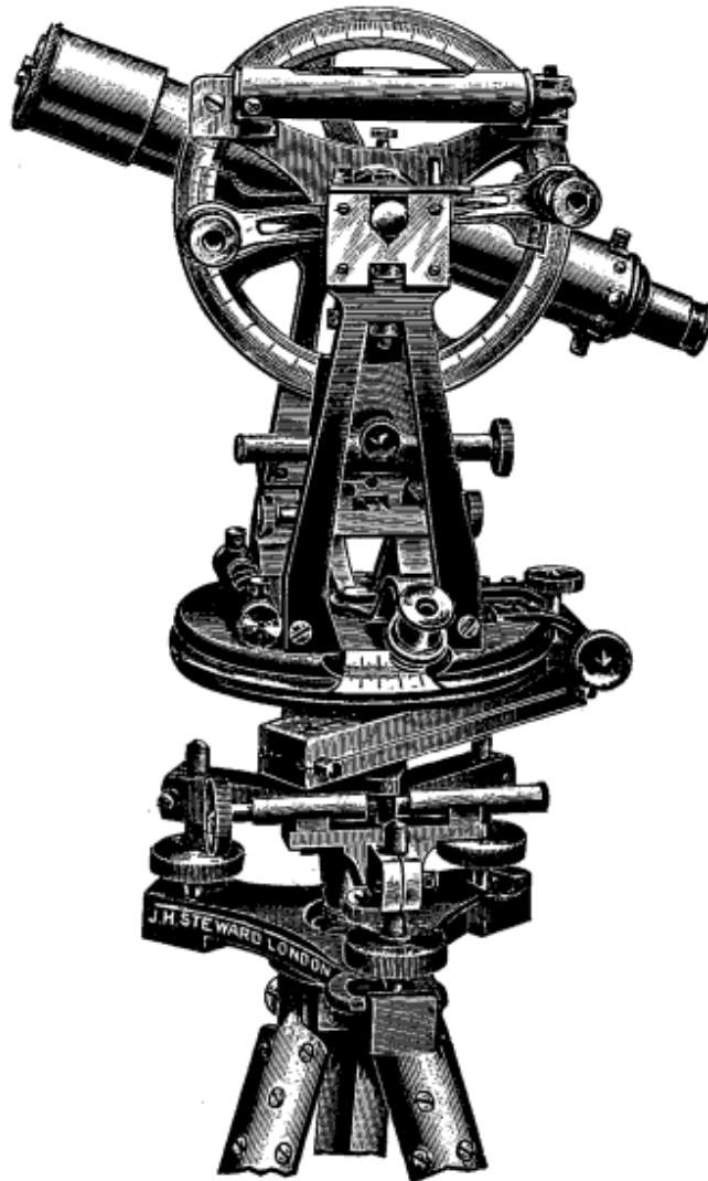
Transit Theodolite. FIG. 2.
