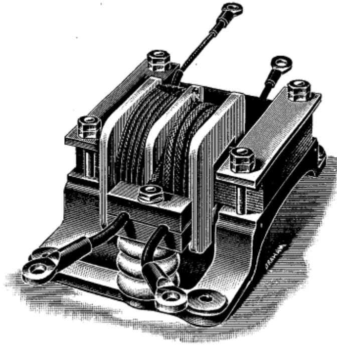
Series Transformer. FIG. 10.
