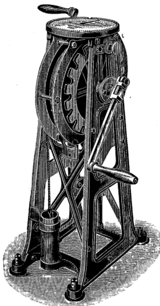
Sounding Machine. FIG. 1.
