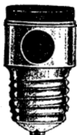
WE1483. Swivel socket. Can be used on any standard socket lamp, enables the operator to adjust the clear space of ophthalmic lamp without breaking the contact.
