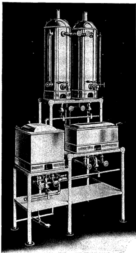
W.C. 1549 The D. T. Vail Pyramid Sterilizing Outfit for Water, Instruments and Utensils.
