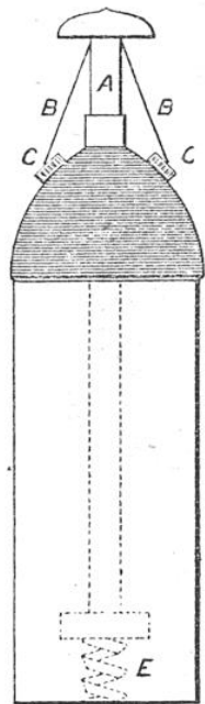
PROJECTILE LUDWIG A BRIQUET
