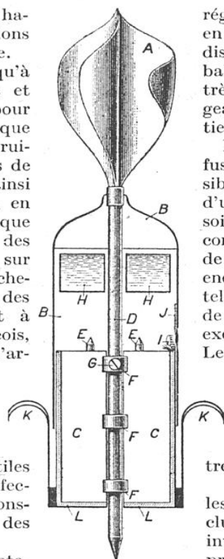
PROJECTILE A EMPENNE
