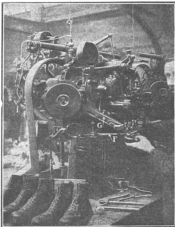
MACHINE A MONTER LE BOUT
