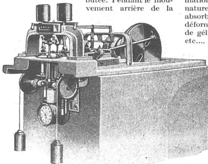
MACHINE A USER LES LIMES
