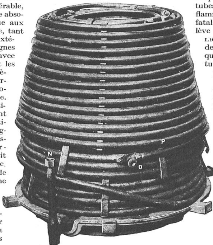
CHAUDIÈRE DE L'AUTOMOBILE NEWCOMB AND SCOTT
