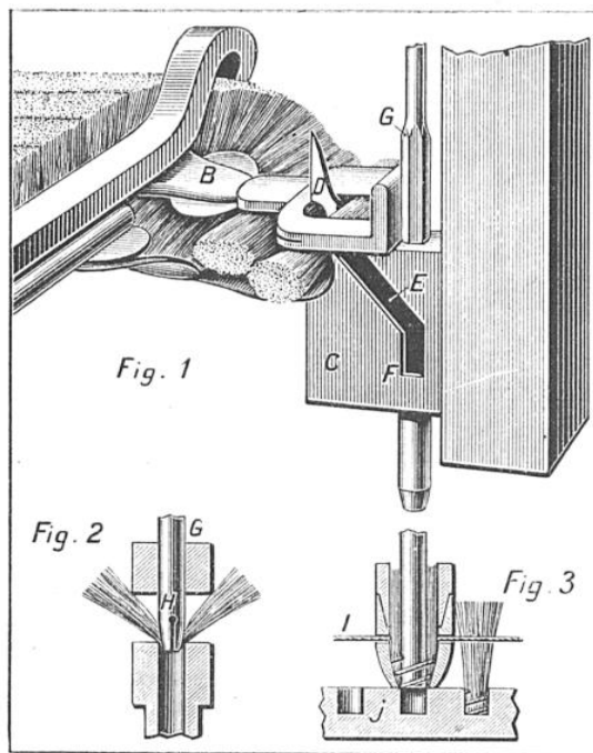
MACHINE A MONTER DE M. WOODBURY
