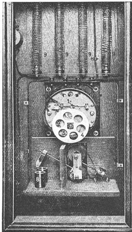
FIG. 9. — RELAIS A MERCURE
