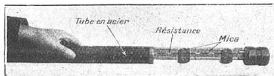
FIG. 5. — TUBE CHAUFFANT
