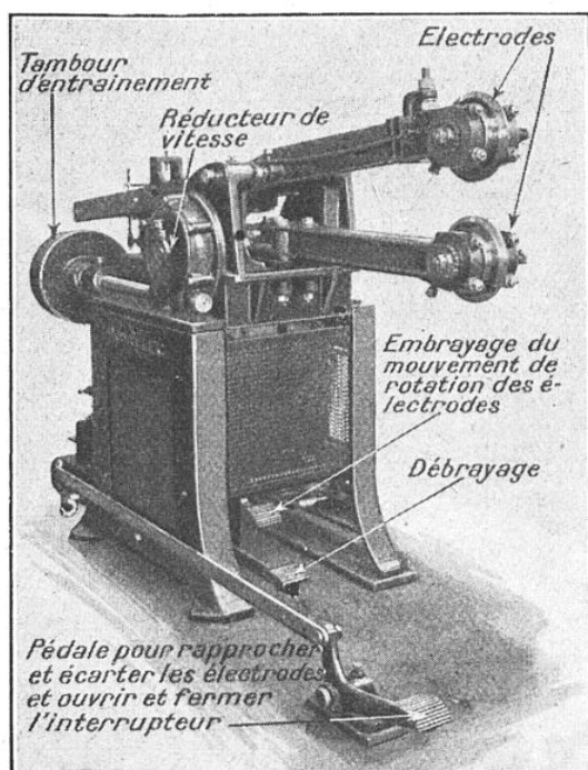
FIG. 4. — MACHINE A SOUDER CONTINUE
